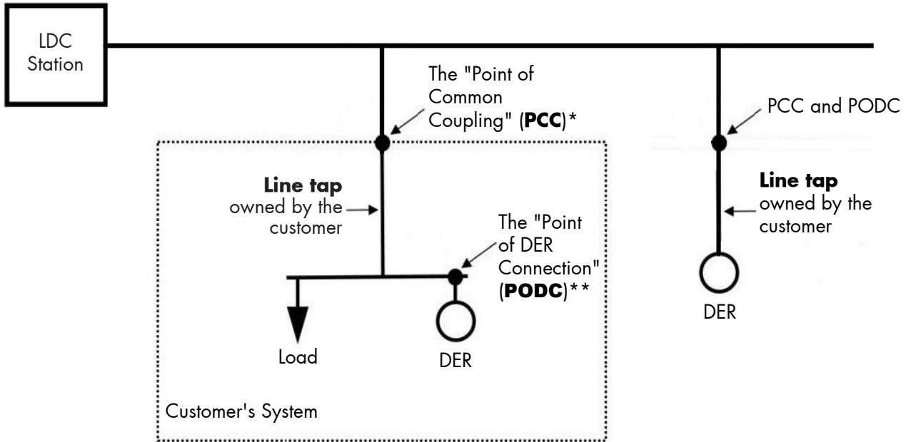
Figure A1: Where There is No New InnPower Corporation Owned Line Expansion
